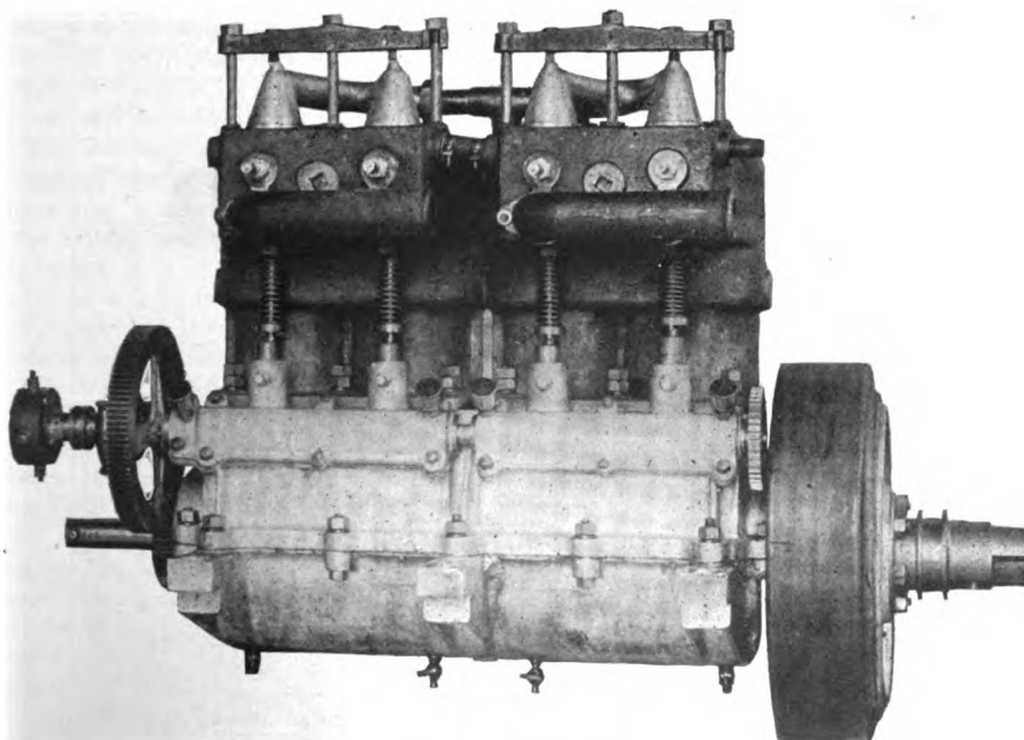
FOUR CYLINDER FIVE-BY-FIVE MOTOR OF ROYAL TOURING CAR.
